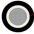
Tinned Copper Clad Aluminium Alloy (Multistranded Flexible) Insulation - XLPO (EBXL) Outer Sheath - XLPO (EBXL) - Black
