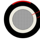
Tinned Copper Clad Aluminium Alloy (Multistranded Flexible) Insulation - XLPO (EBXL) Outer Sheath - XLPO (EBXL) - Black with Red Strip
